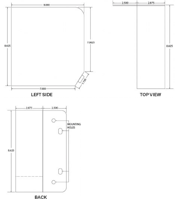
Wall Mount Cable Retractor Dimensional Drawings
