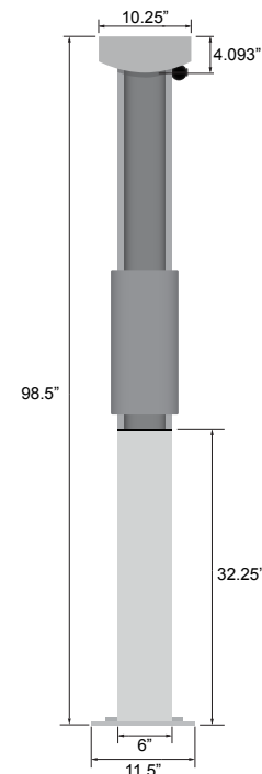
Dimensional Drawing
