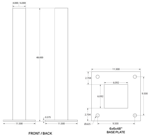
Dimensional Drawings (dimensions in inches)
