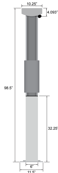
Dimensional Drawing
