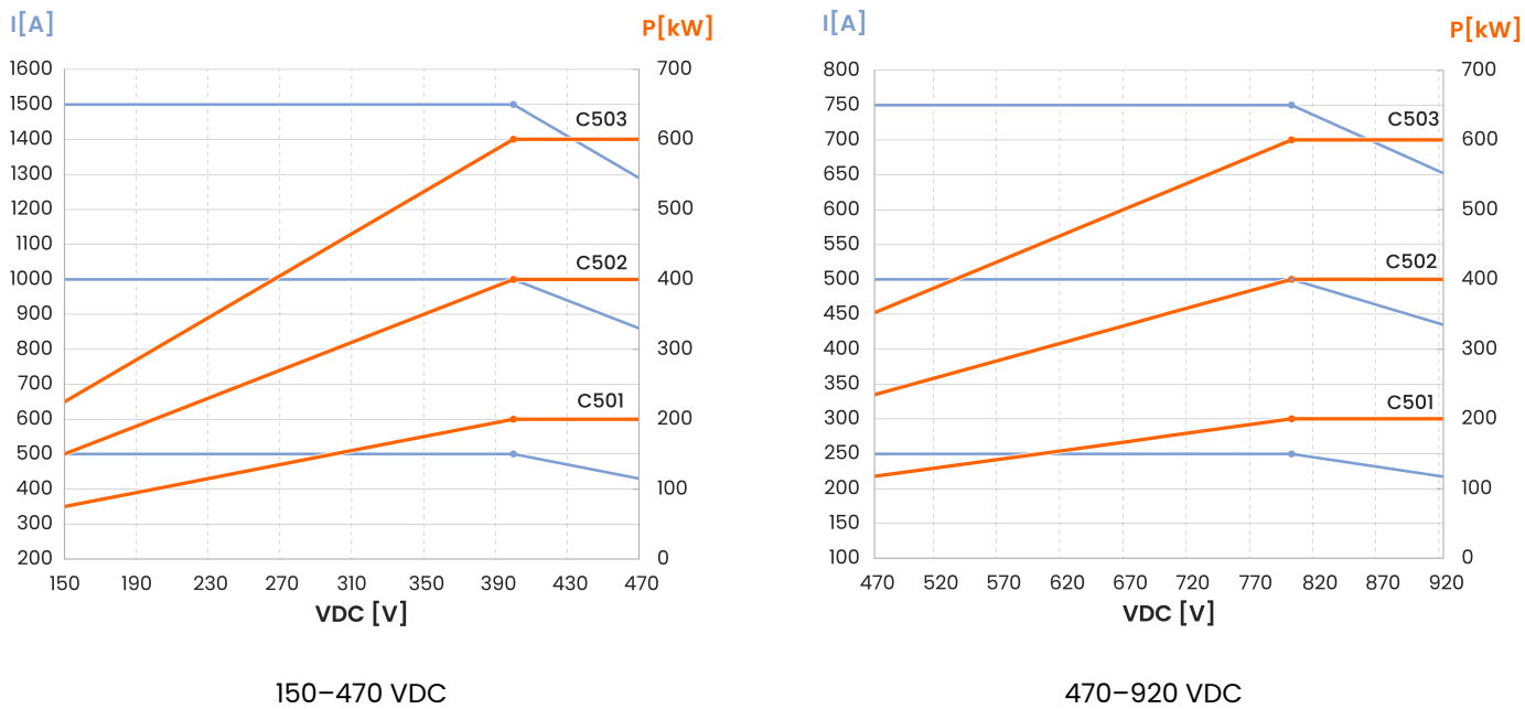
Figure 1. Power curve – standard operation
