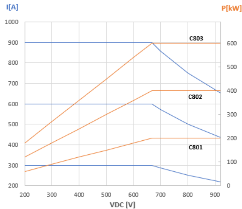
Figure 1. Power curve – standard operation
