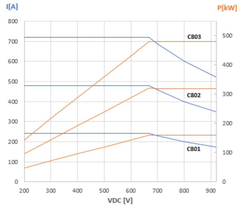
Figure 2. Power curve – continuous operation
